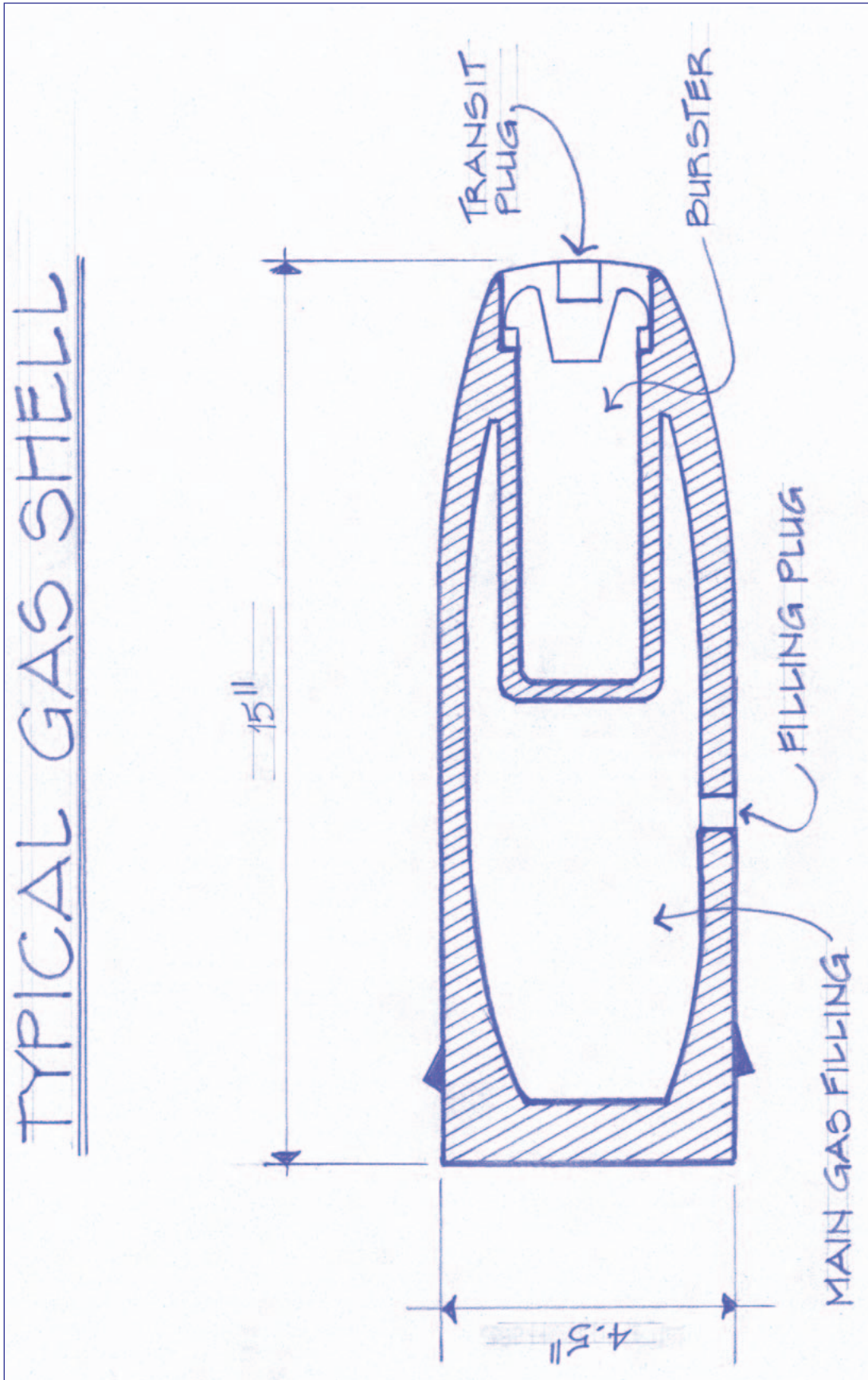
Poison Gas Shell Diagram
